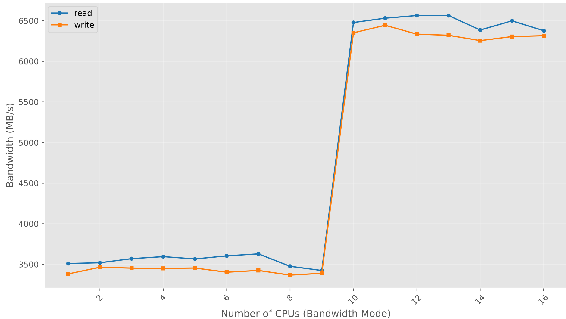
Bandwidth vs Number of CPUs (Bandwidth Mode)
